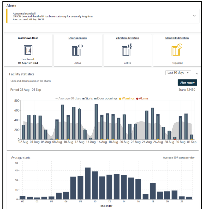
Individual lift performance statistics – Starts
